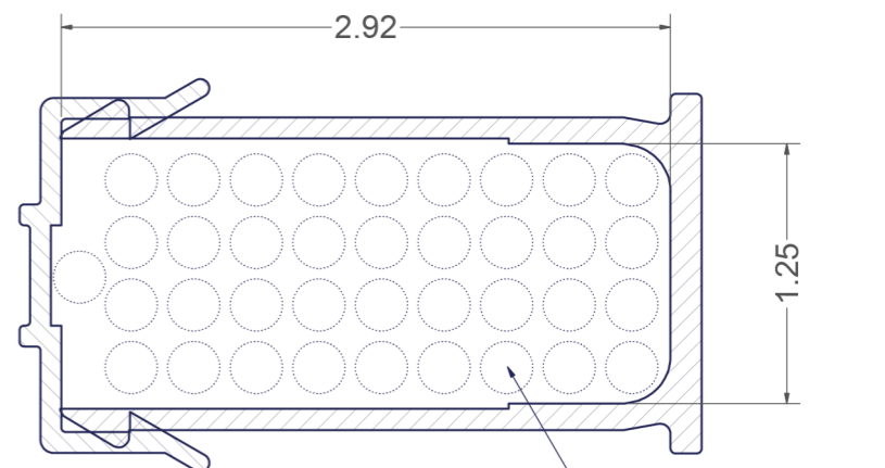
SECTION A-A SCALE 2 37X Ø.25 CABLE 50% FILL SHOWN
